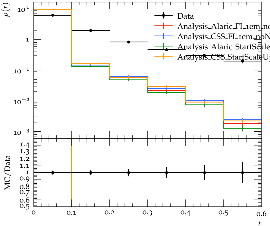
Jet shape \rho for p_{\perp} \in 110\text{--}160 GeV, y \in 0.3\text{--}0.8
