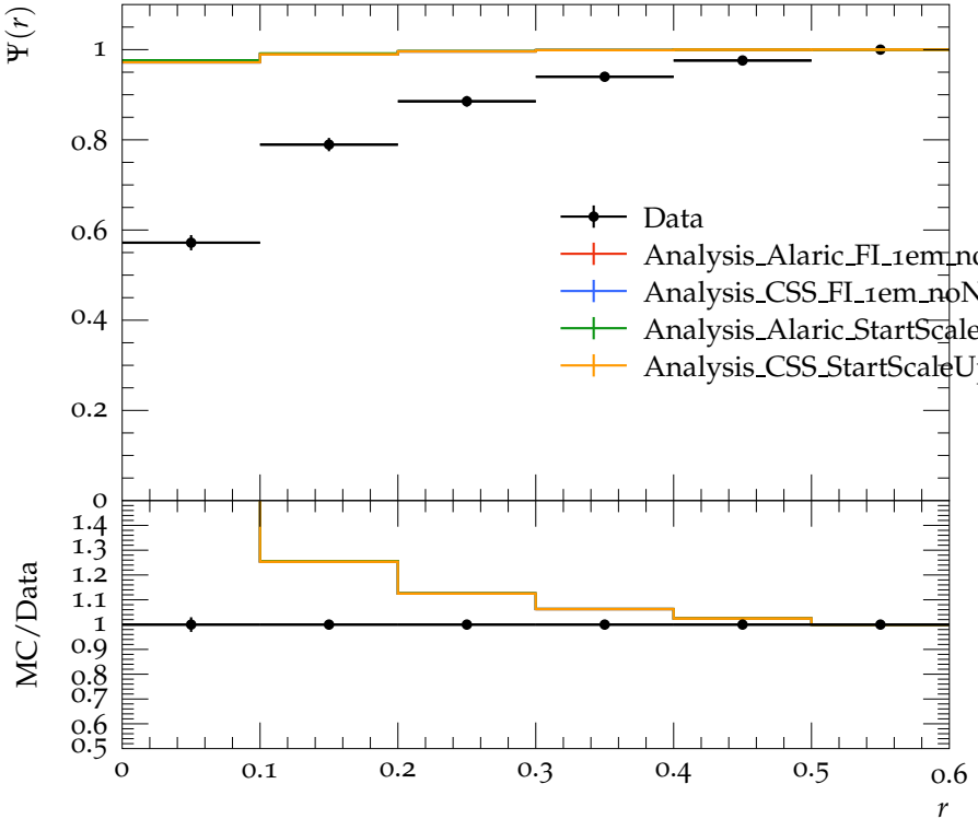
Jet shape \Psi for p_{\perp} \in 80\text{--}110\text{ GeV} , y \in 0.0\text{--}2.8
