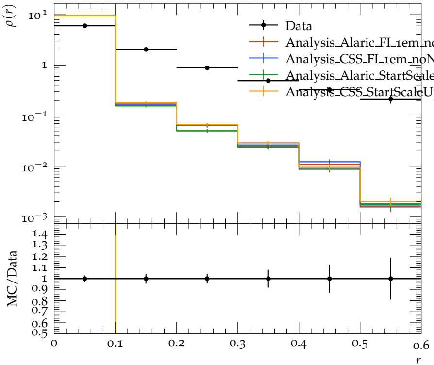
Jet shape \rho for p_{\perp} \in 80\text{--}110\text{ GeV} , y \in 2.1\text{--}2.8
