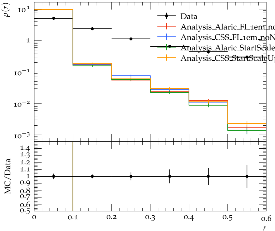
Jet shape \rho for p_{\perp} \in 60\text{--}80\text{ GeV} , y \in 0.0\text{--}0.3
