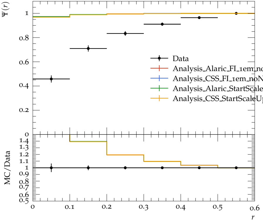
Jet shape \Psi for p_{\perp} \in 40\text{--}60\text{ GeV} , y \in 2.1\text{--}2.8
