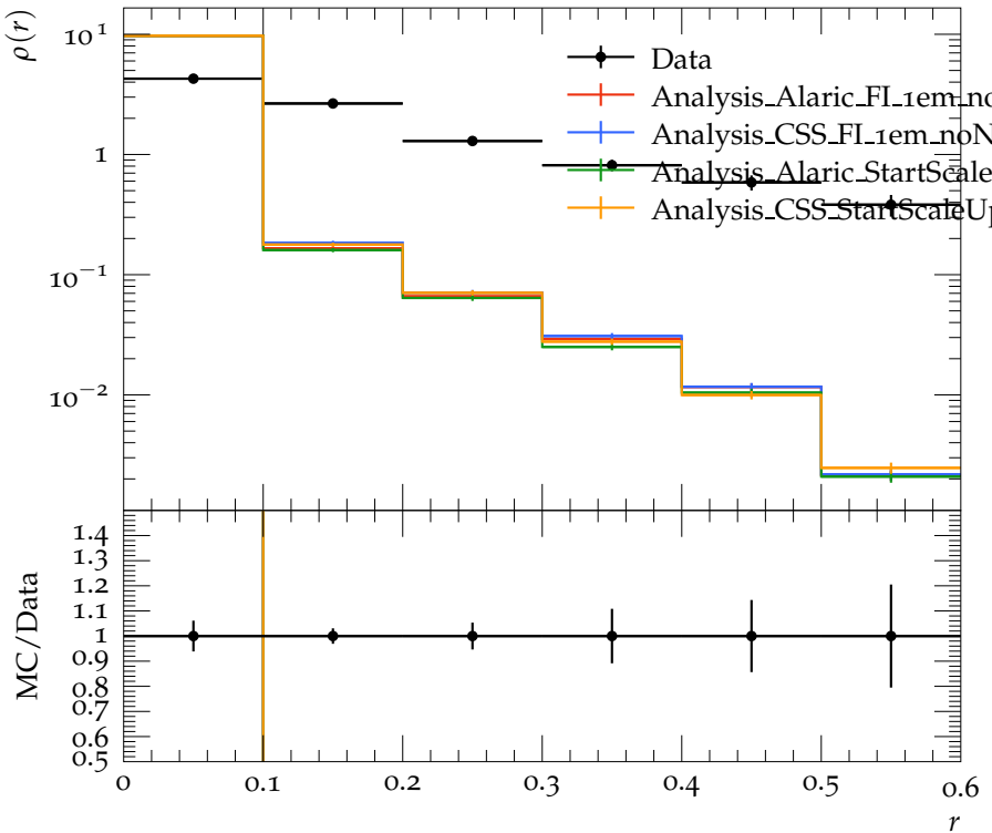
Jet shape \rho for p_{\perp} \in 40\text{--}60\text{ GeV} , y \in 0.3\text{--}0.8
