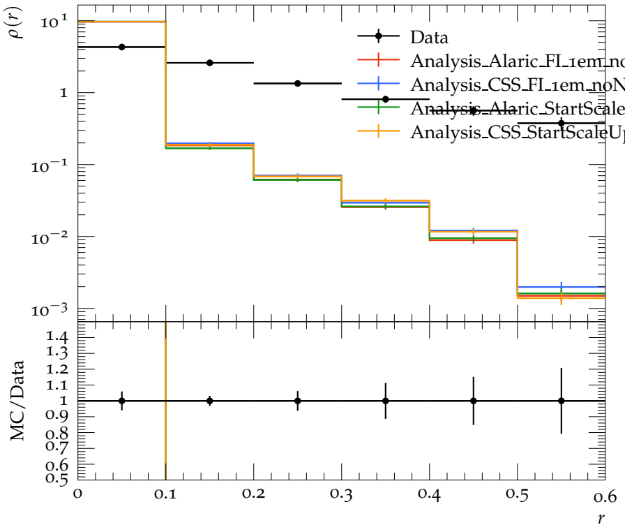
Jet shape \rho for p_{\perp} \in 40\text{--}60\text{ GeV} , y \in 0.0\text{--}0.3
