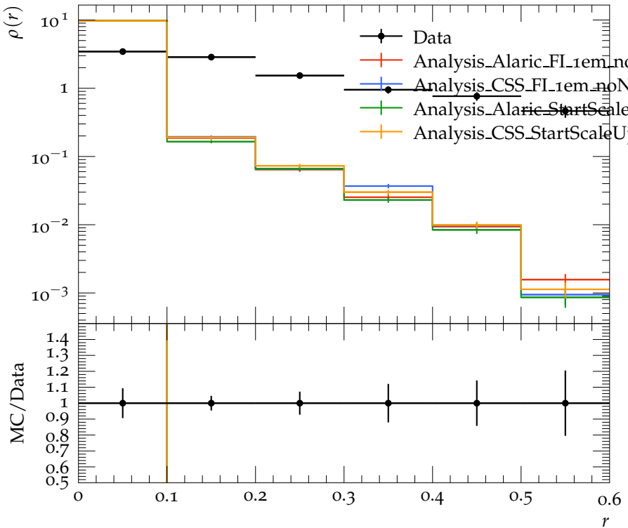
Jet shape \rho for p_{\perp} \in 30\text{--}40\text{ GeV} , y \in 0.0\text{--}0.3
