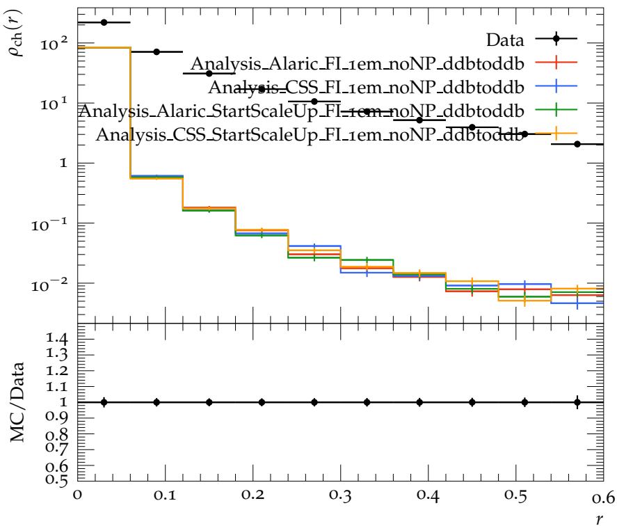
Density of charged particles for 110 \text{ GeV} < p_{T \text{ jet}} < 160 \text{ GeV}
