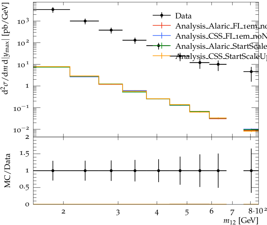
Dijet mass spectrum for 0.3 < |y_{\max}| < 0.8 . anti-KT, R = 0.6 .
