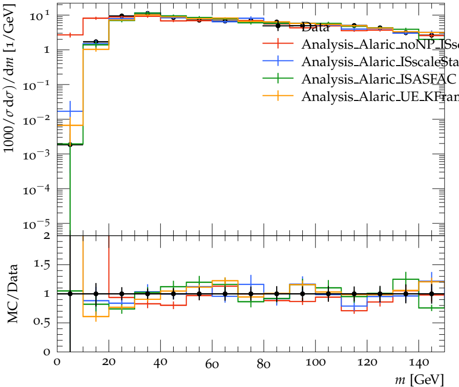
Trimmed AK7 dijets, (p_T^1 + p_T^2)/2 = 1000\text{--}1500 GeV
