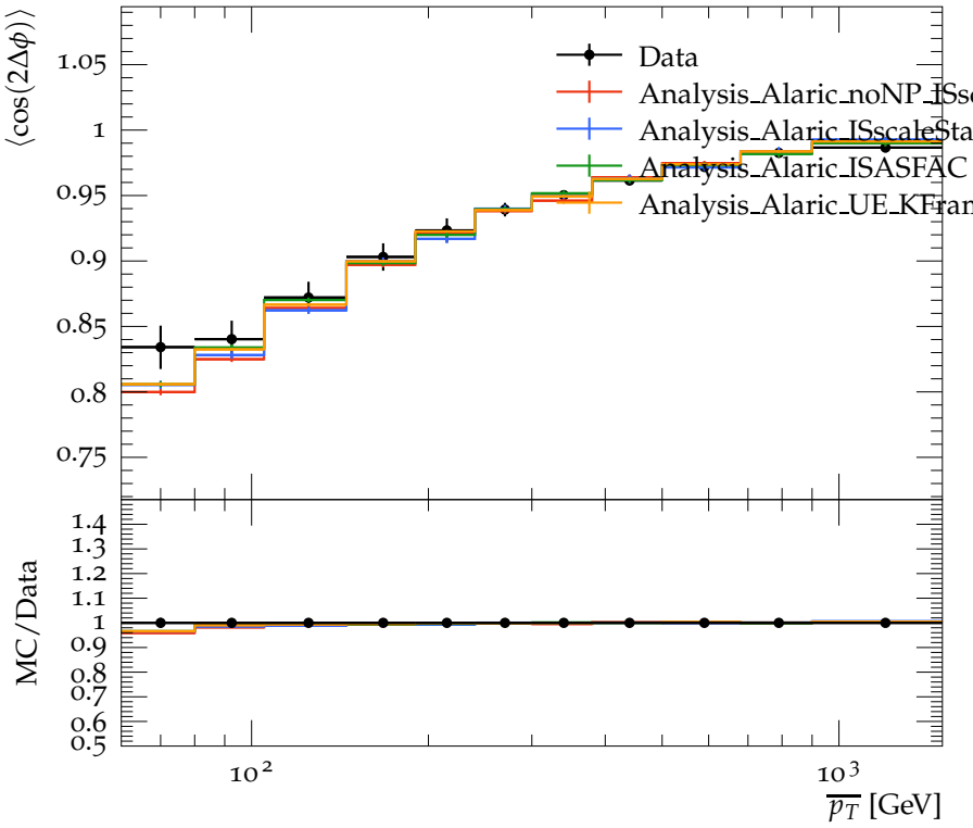
\langle \cos(2\Delta\phi) \rangle for gap events as a function of \overline{p_T}
