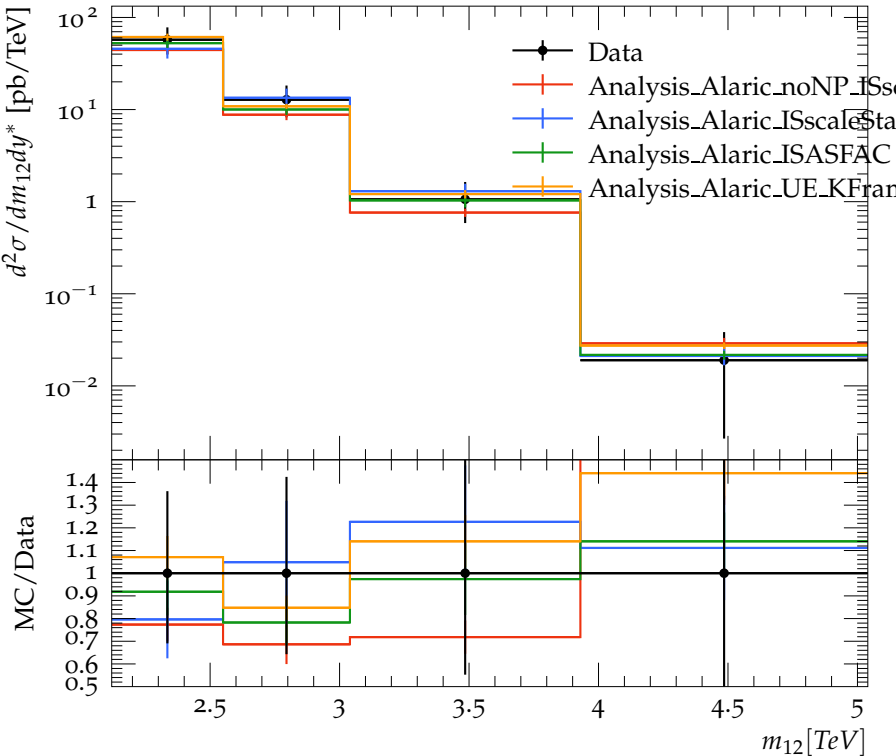
Dijet double-differential cross sections ( 2.5 < y^* < 3.0 ), R=0.4
