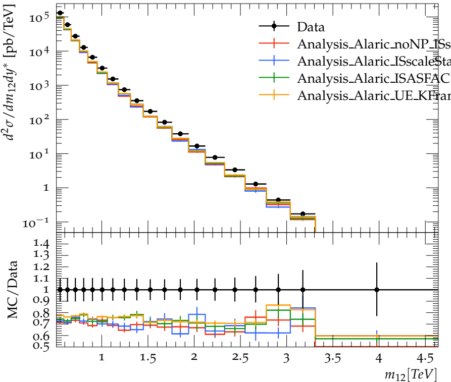
Dijet double-differential cross sections ( 1.0 < y^* < 1.5 ), R=0.4
