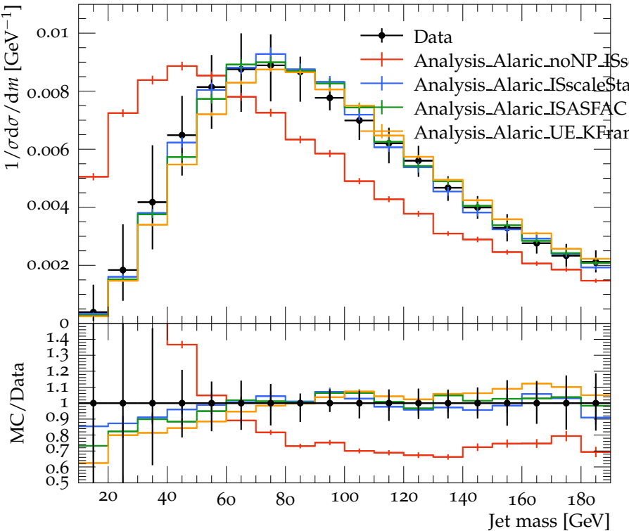
Cambridge-Aachen jets, R=1.2 , 300 \text{ GeV} < p_{\perp} < 400 \text{ GeV}
