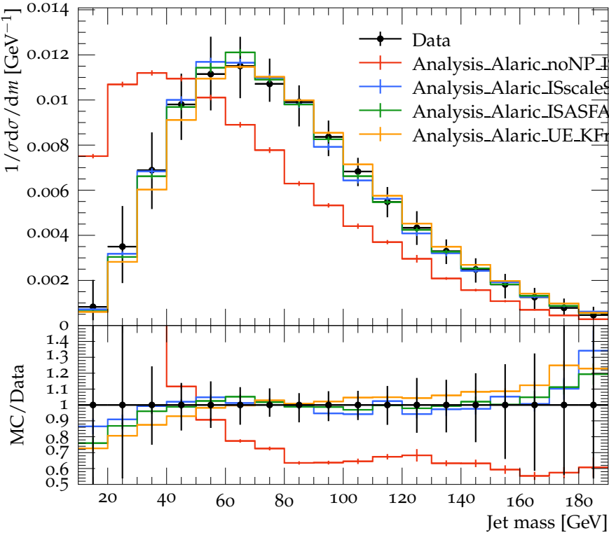
Cambridge-Aachen jets, R=1.2 , 200 \text{ GeV} < p_{\perp} < 300 \text{ GeV}
