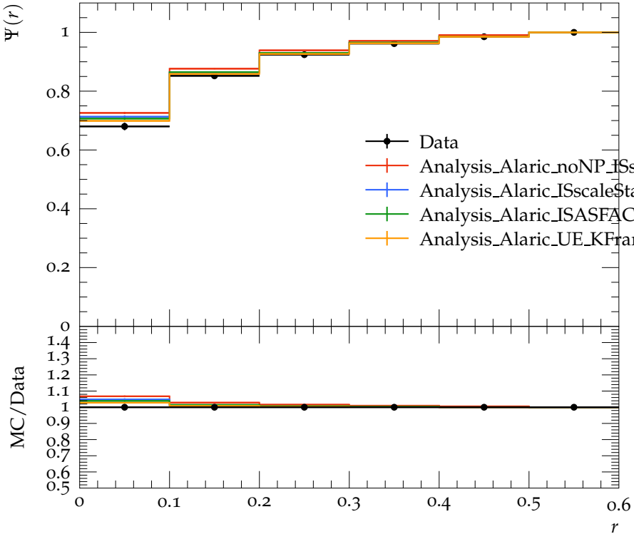
Jet shape \Psi for p_{\perp} \in 210\text{--}260\text{ GeV} , y \in 0.0\text{--}0.3
