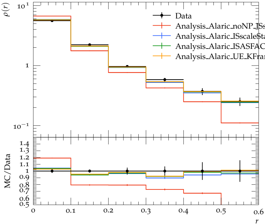
Jet shape \rho for p_{\perp} \in 80\text{--}110\text{ GeV} , y \in 0.0\text{--}0.3
