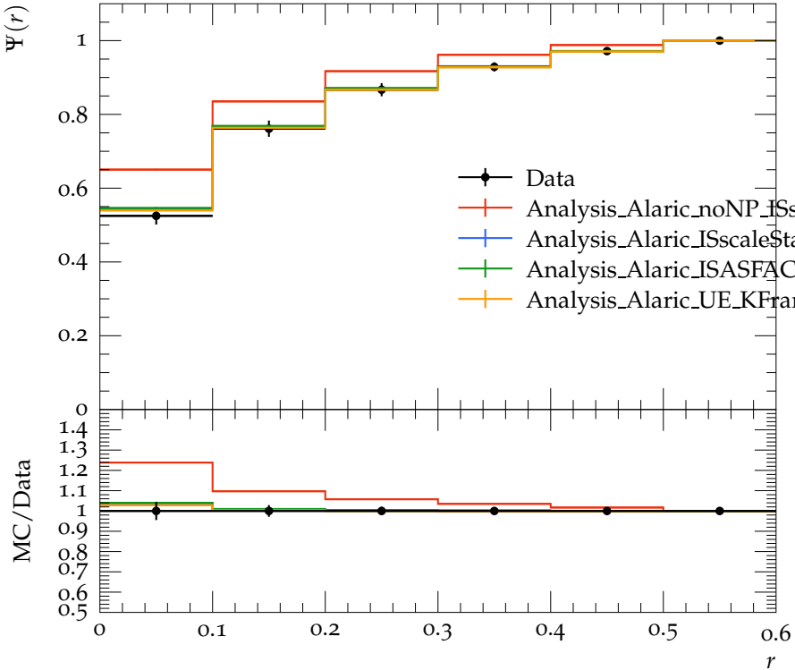
Jet shape \Psi for p_{\perp} \in 60\text{--}80\text{ GeV} , y \in 1.2\text{--}2.1
