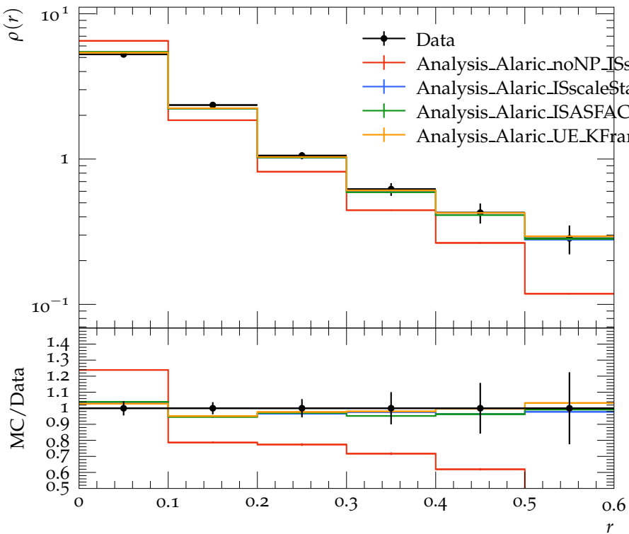
Jet shape \rho for p_{\perp} \in 60\text{--}80\text{ GeV} , y \in 1.2\text{--}2.1
