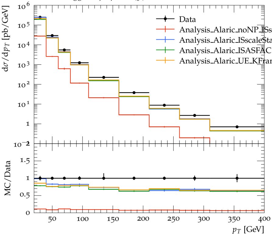
Lifetime tagged b -jet p_T for |y| < 2.1 , anti- k_T , R = 0.4 .
