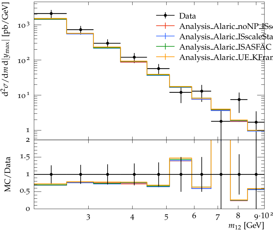
Dijet mass spectrum for 0.8 < |y_{\max}| < 1.2 . anti-KT, R = 0.4 .
