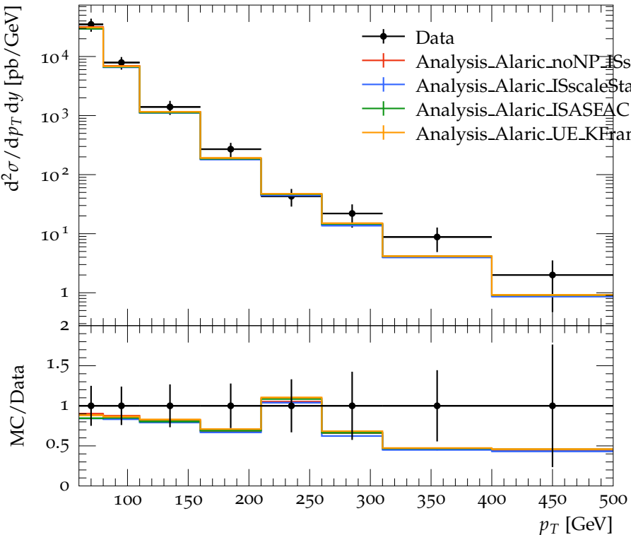
Inclusive jet p_T spectrum for |y| < 0.3 . anti-KT, R = 0.4 .
