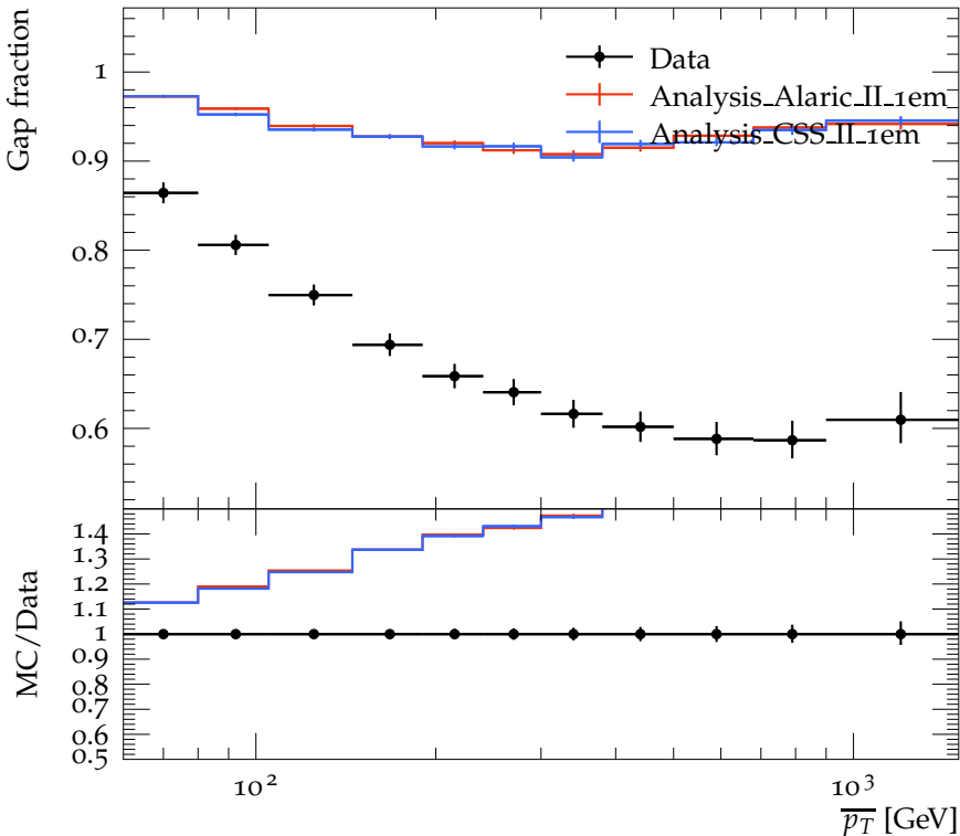
Gap fraction as a function of leading dijet scalar mean p_T
