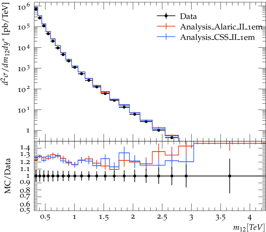
Dijet double-differential cross sections ( 0.5 < y^* < 1.0 ), R=0.4
