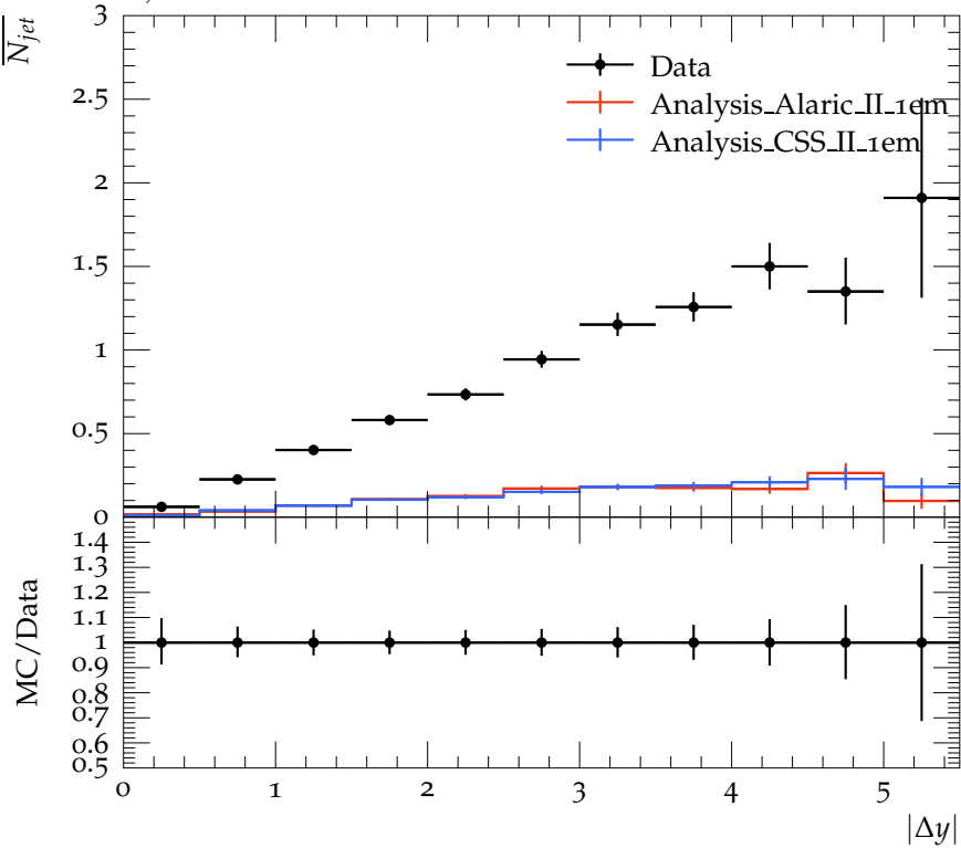
\overline{N}_{jet} vs |\Delta y| for 210 < \overline{P}_T < 240 , Leading Jet
