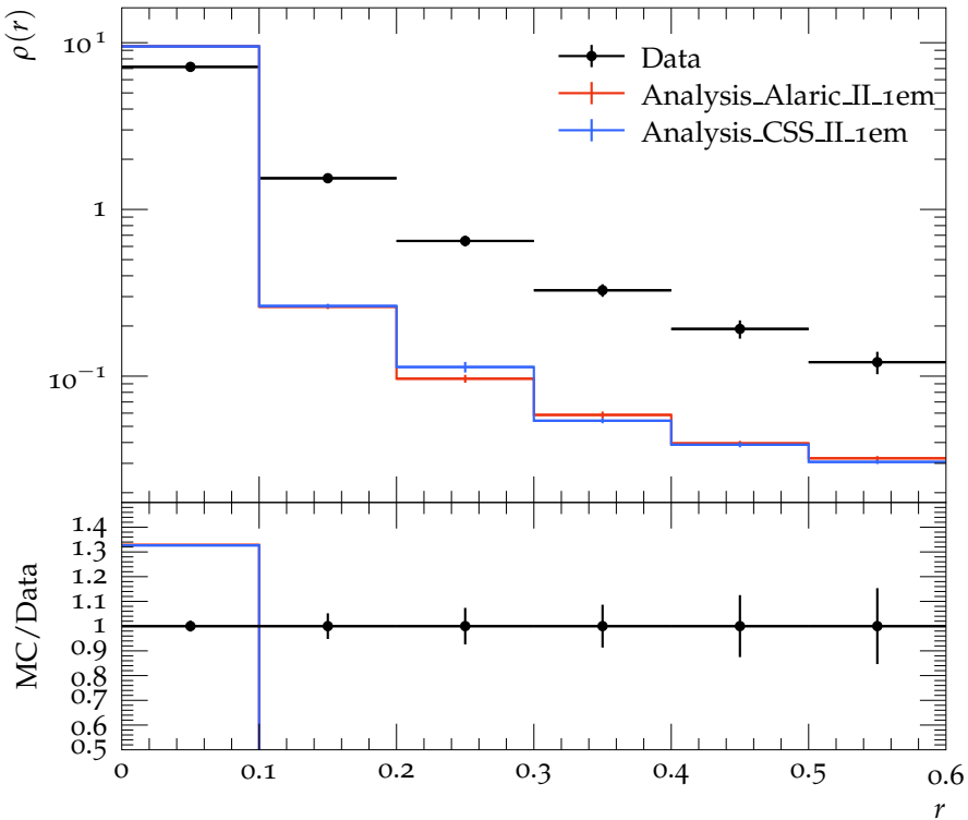
Jet shape \rho for p_{\perp} \in 260\text{--}310 GeV, y \in 0.8\text{--}1.2
