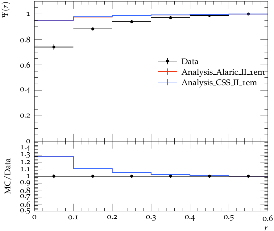
Jet shape \Psi for p_{\perp} \in 210\text{--}260\text{ GeV} , y \in 2.1\text{--}2.8
