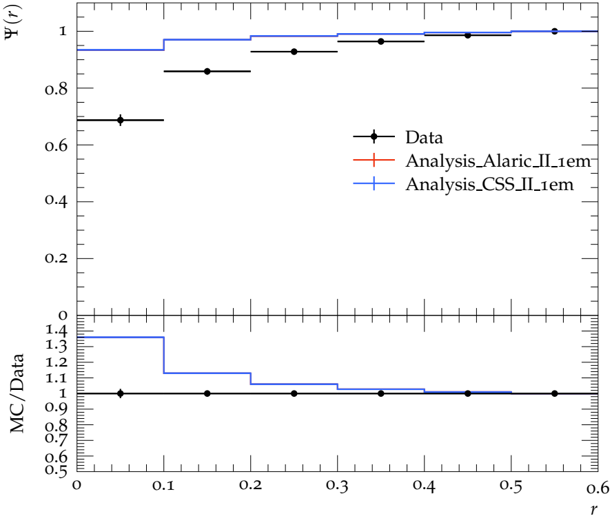
Jet shape \Psi for p_{\perp} \in 210\text{--}260 GeV, y \in 0.3\text{--}0.8
