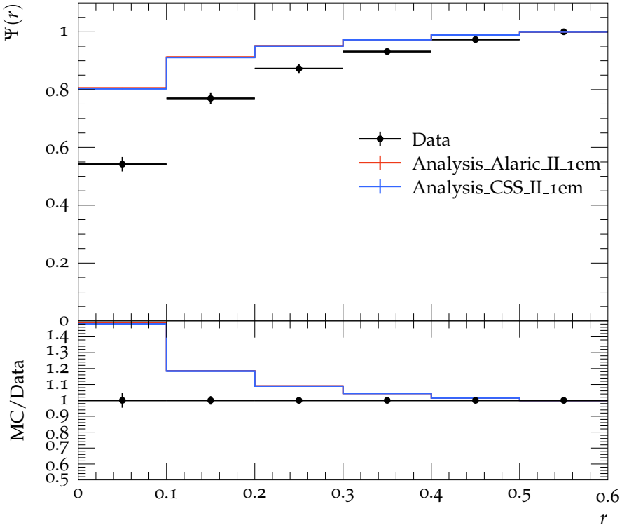
Jet shape \Psi for p_{\perp} \in 60\text{--}80\text{ GeV} , y \in 2.1\text{--}2.8
