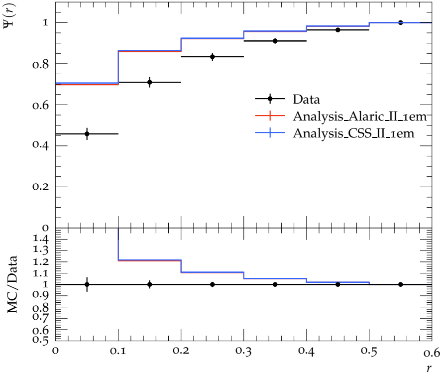
Jet shape \Psi for p_{\perp} \in 40\text{--}60\text{ GeV} , y \in 2.1\text{--}2.8
