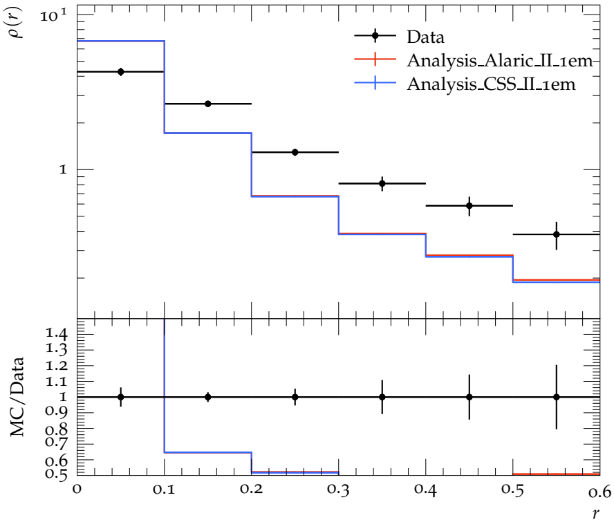
Jet shape \rho for p_{\perp} \in 40\text{--}60\text{ GeV} , y \in 0.3\text{--}0.8
