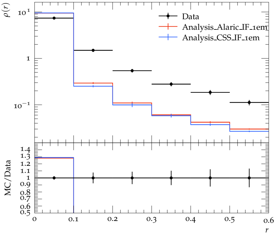
Jet shape \rho for p_{\perp} \in 310\text{--}400 GeV, y \in 0.0\text{--}0.3
