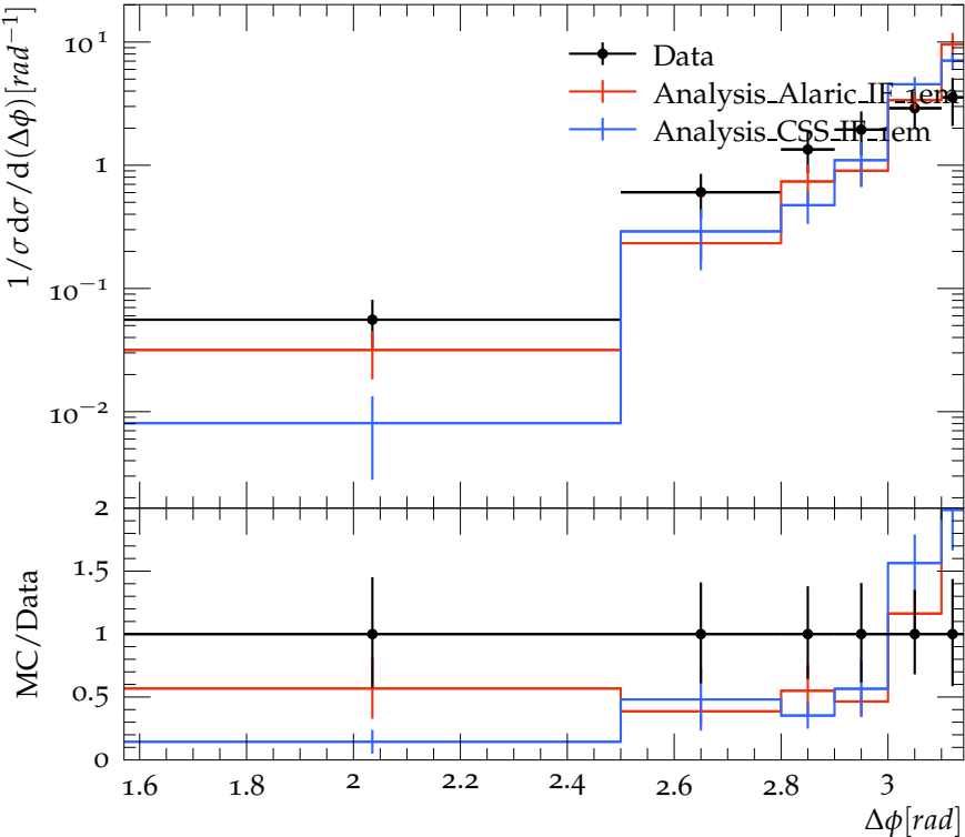
Dijet \Delta\phi for m_{jj} > 110 GeV, anti- k_T , R = 0.4
