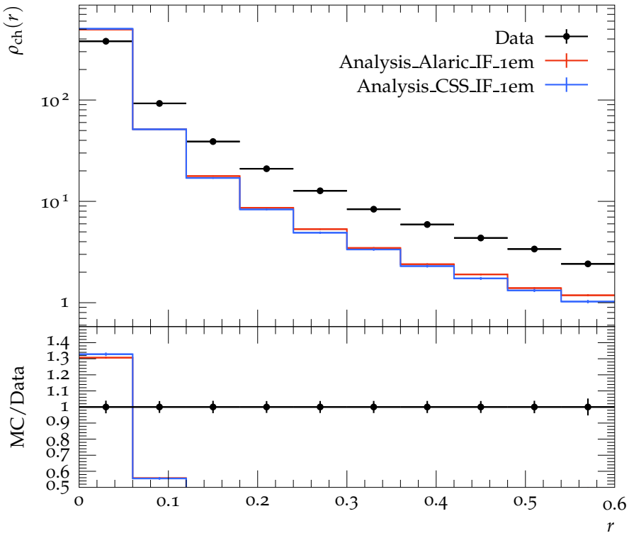
Density of charged particles for 260 \text{ GeV} < p_{T \text{ jet}} < 310 \text{ GeV}
