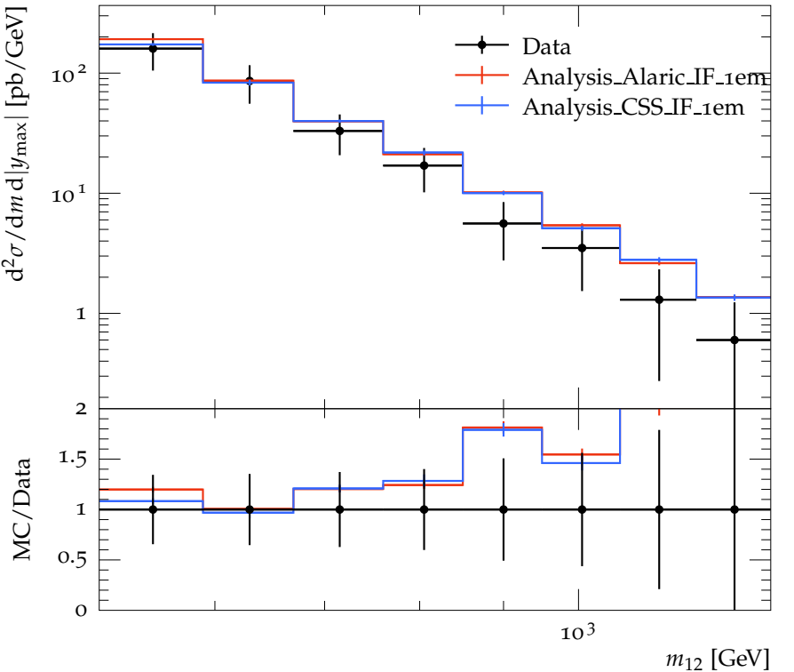
Dijet mass spectrum for 1.2 < |y_{\max}| < 2.1 . anti-KT, R = 0.6 .
