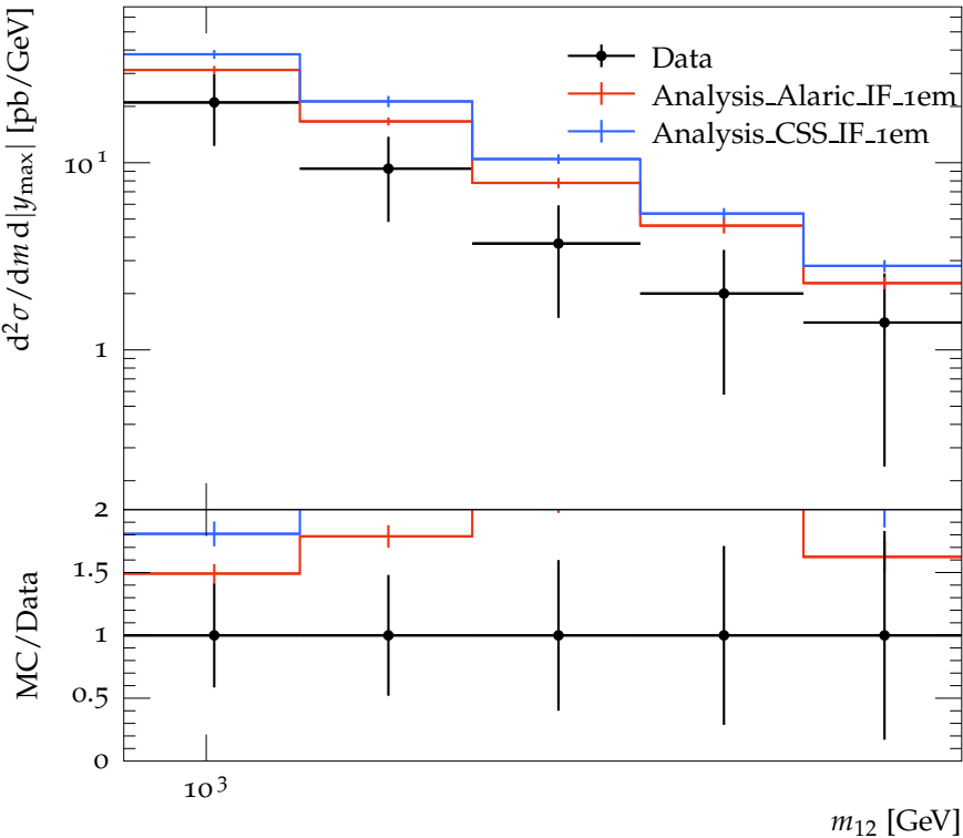
Dijet mass spectrum for 2.1 < |y_{\max}| < 2.8 . anti-KT, R = 0.4 .
