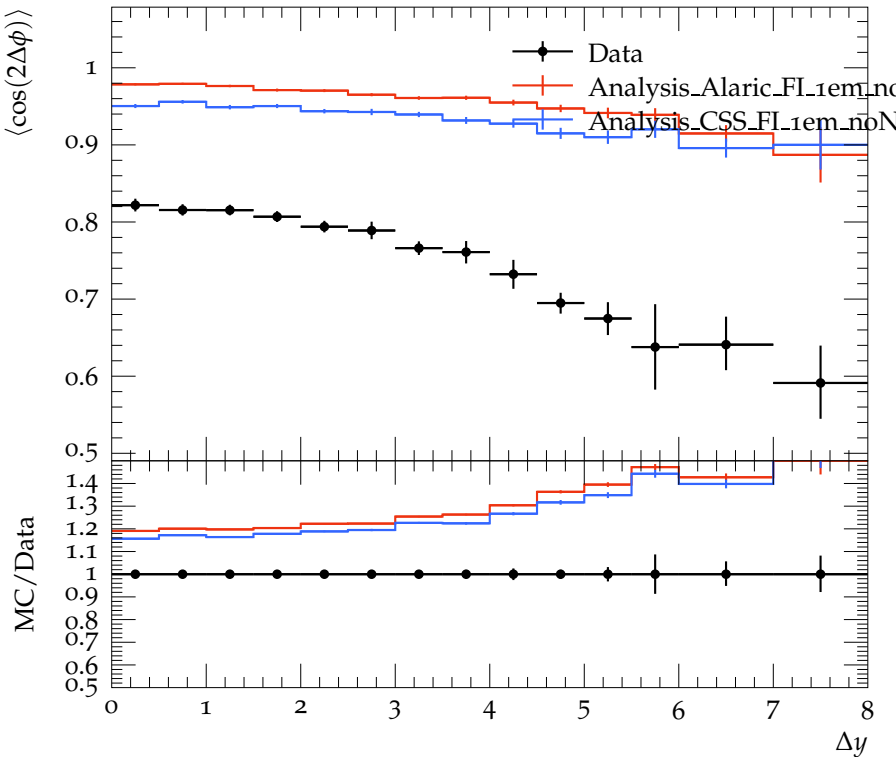
\langle \cos(2\Delta\phi) \rangle for inclusive events as a function of \Delta\gamma
