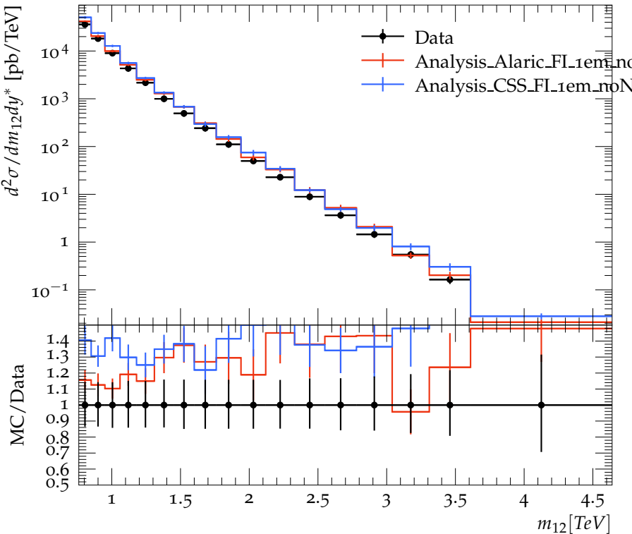
Dijet double-differential cross sections ( 1.5 < y^* < 2.0 ), R=0.4
