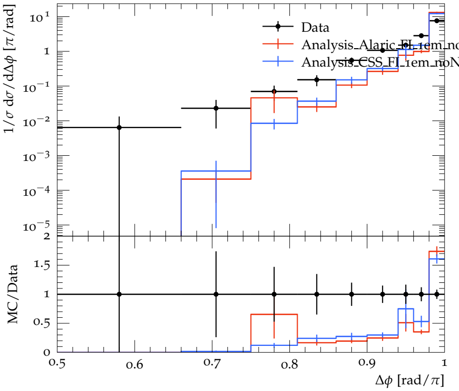
Dijet azimuthal decorrelations for 600 < p_{\perp}^{\text{max}}/\text{GeV} < 800
