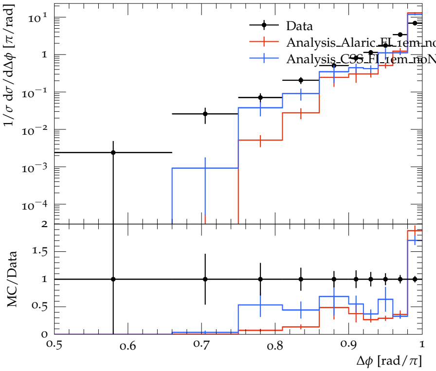
Dijet azimuthal decorrelations for 500 < p_{\perp}^{\text{max}}/\text{GeV} < 600
