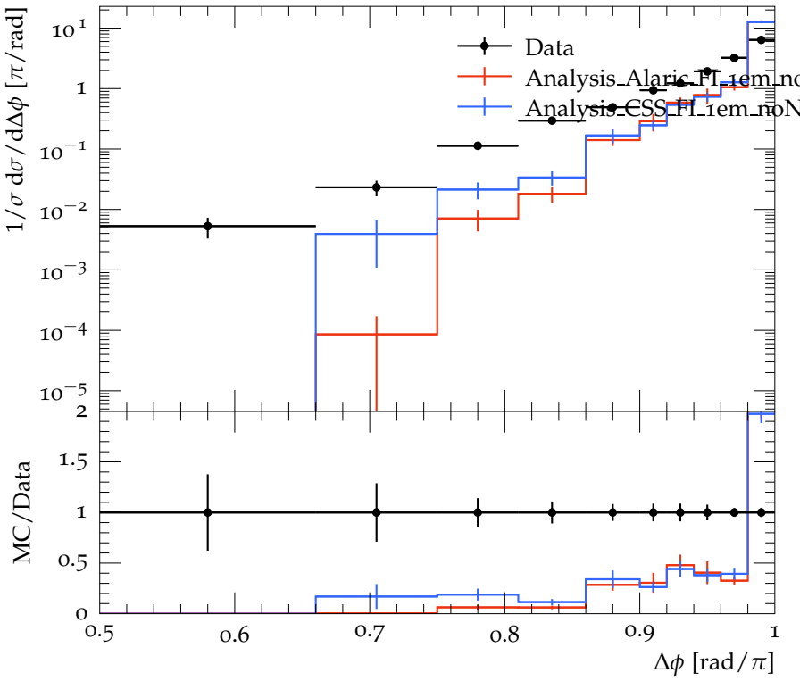
Dijet azimuthal decorrelations for 400 < p_{\perp}^{\text{max}}/\text{GeV} < 500
