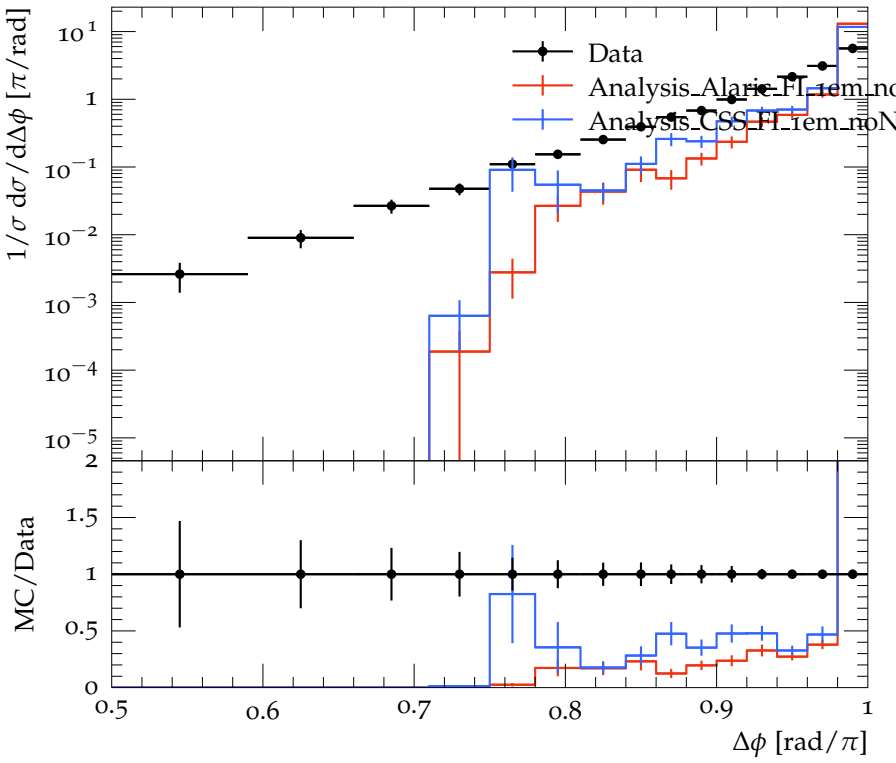
Dijet azimuthal decorrelations for 310 < p_{\perp}^{\text{max}}/\text{GeV} < 400
