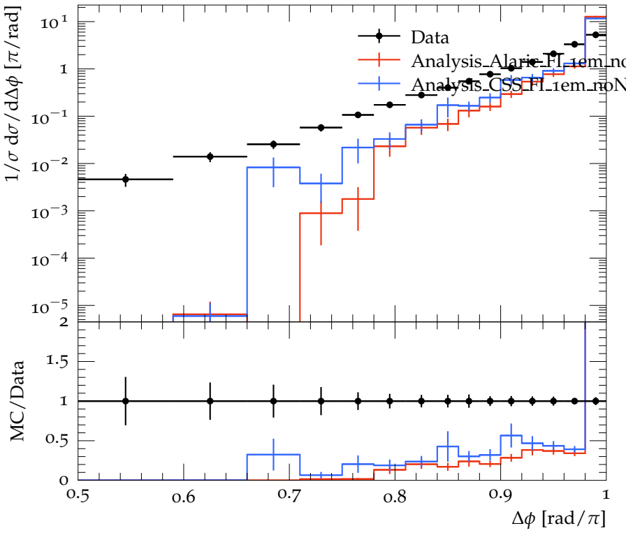
Dijet azimuthal decorrelations for 260 < p_{\perp}^{\text{max}}/\text{GeV} < 310
