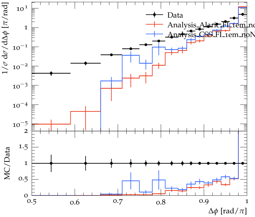
Dijet azimuthal decorrelations for 210 < p_{\perp}^{\text{max}}/\text{GeV} < 260
