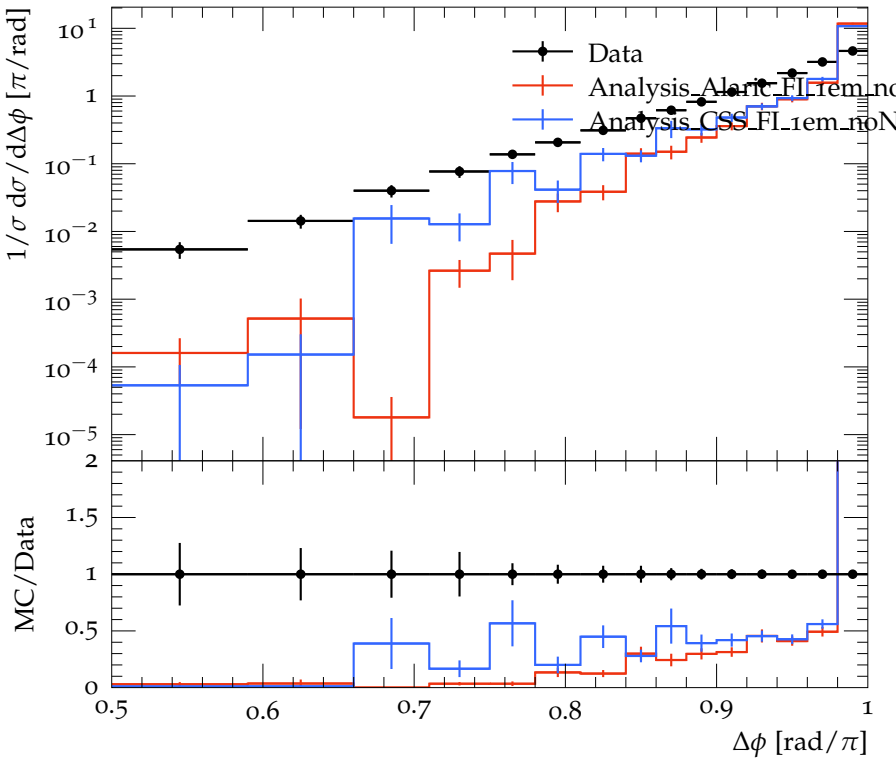
Dijet azimuthal decorrelations for 160 < p_{\perp}^{\text{max}}/\text{GeV} < 210
