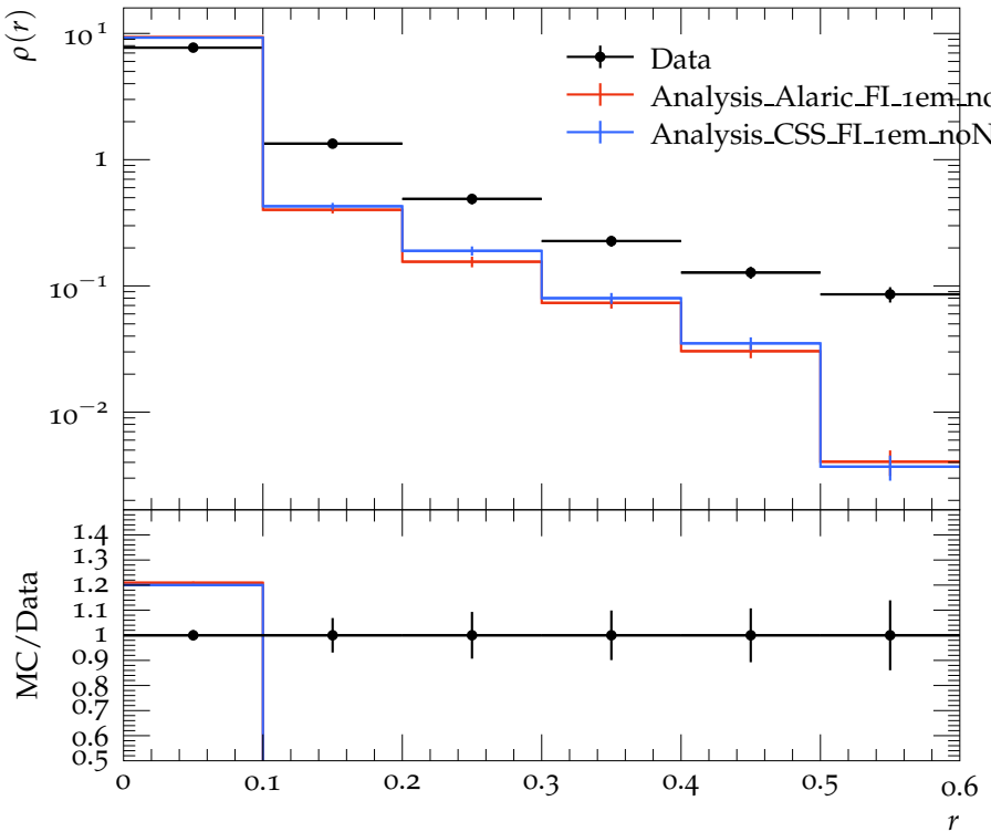
Jet shape \rho for p_{\perp} \in 400\text{--}500 GeV, y \in 0.0\text{--}2.8
