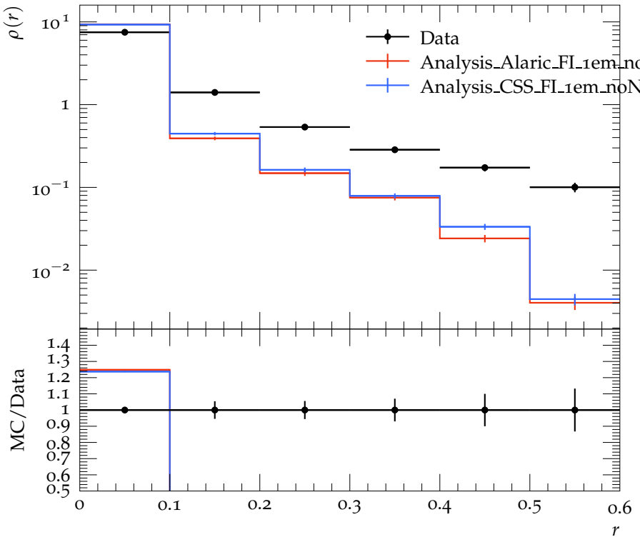
Jet shape \rho for p_{\perp} \in 310\text{--}400 GeV, y \in 0.0\text{--}2.8
