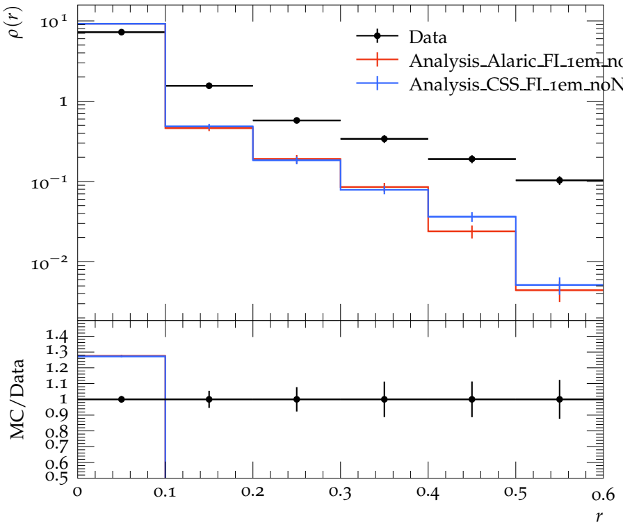
Jet shape \rho for p_{\perp} \in 310\text{--}400 GeV, y \in 0.3\text{--}0.8
