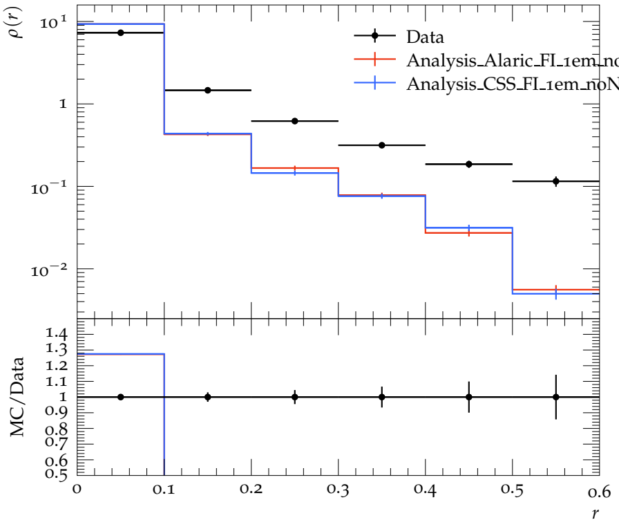
Jet shape \rho for p_{\perp} \in 260\text{--}310 GeV, y \in 0.0\text{--}2.8
